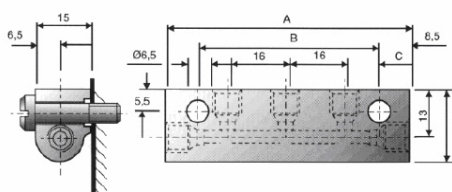
Part No. 42126 5 way double row junction
