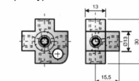
Part No. 42142 (5 way)
