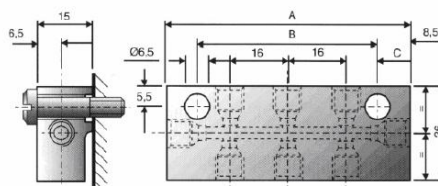
Part No. 42426 8 way double row junction
