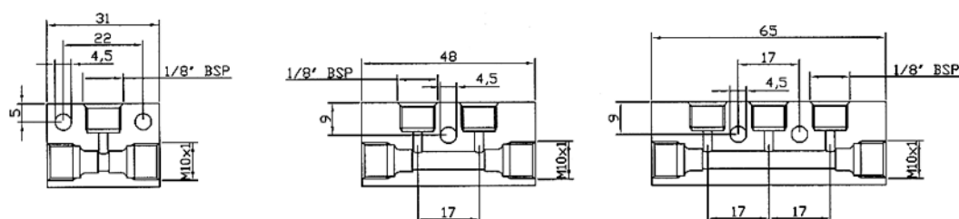
1 Outlet Part Number: 3071301 2 Outlets Part Number: 3071302 3 Outlets Part Number: 3071303
